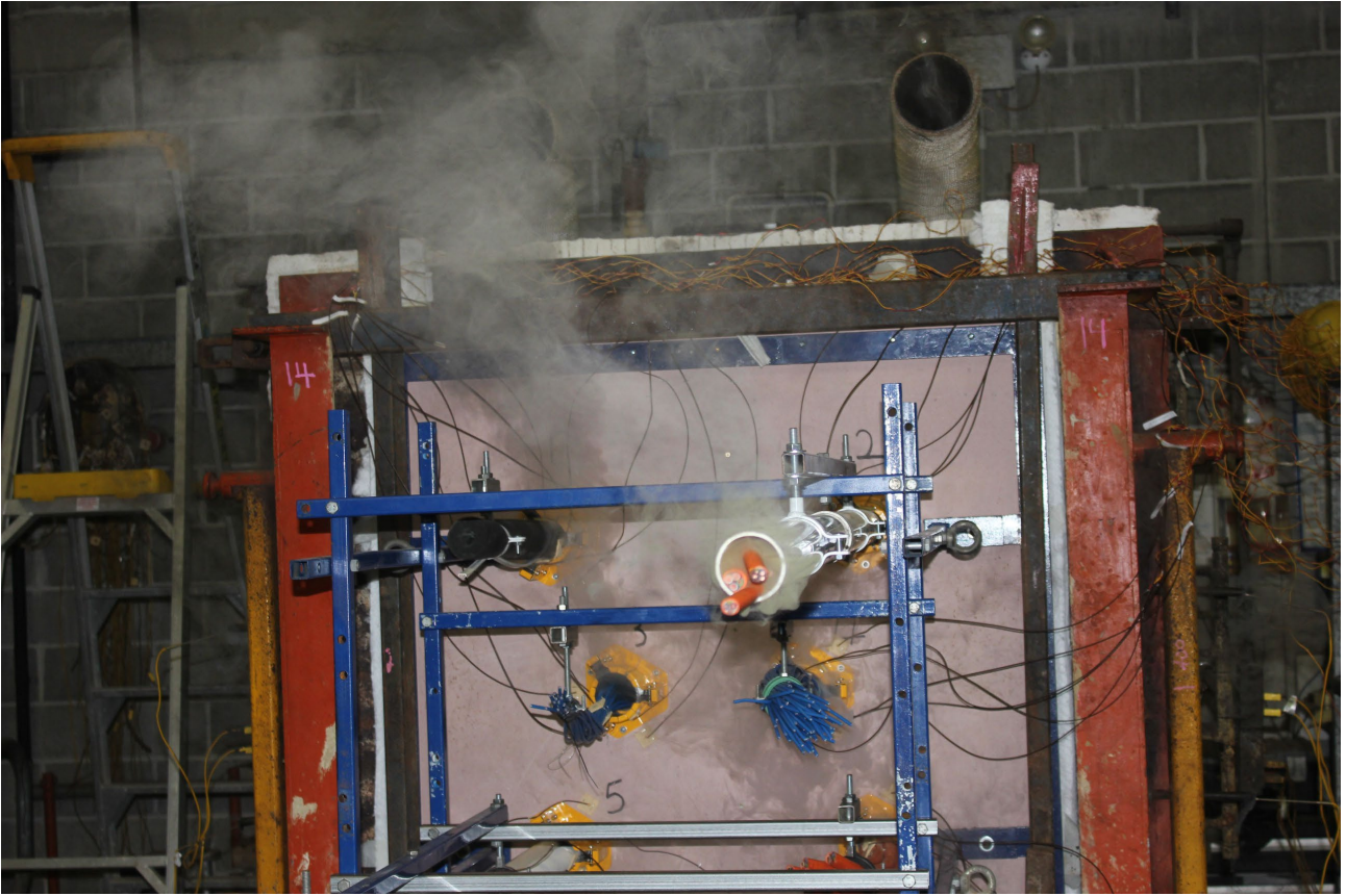
PHOTOGRAPH 3 – SPECIMENS AFTER 2 MINUTES OF TESTING
