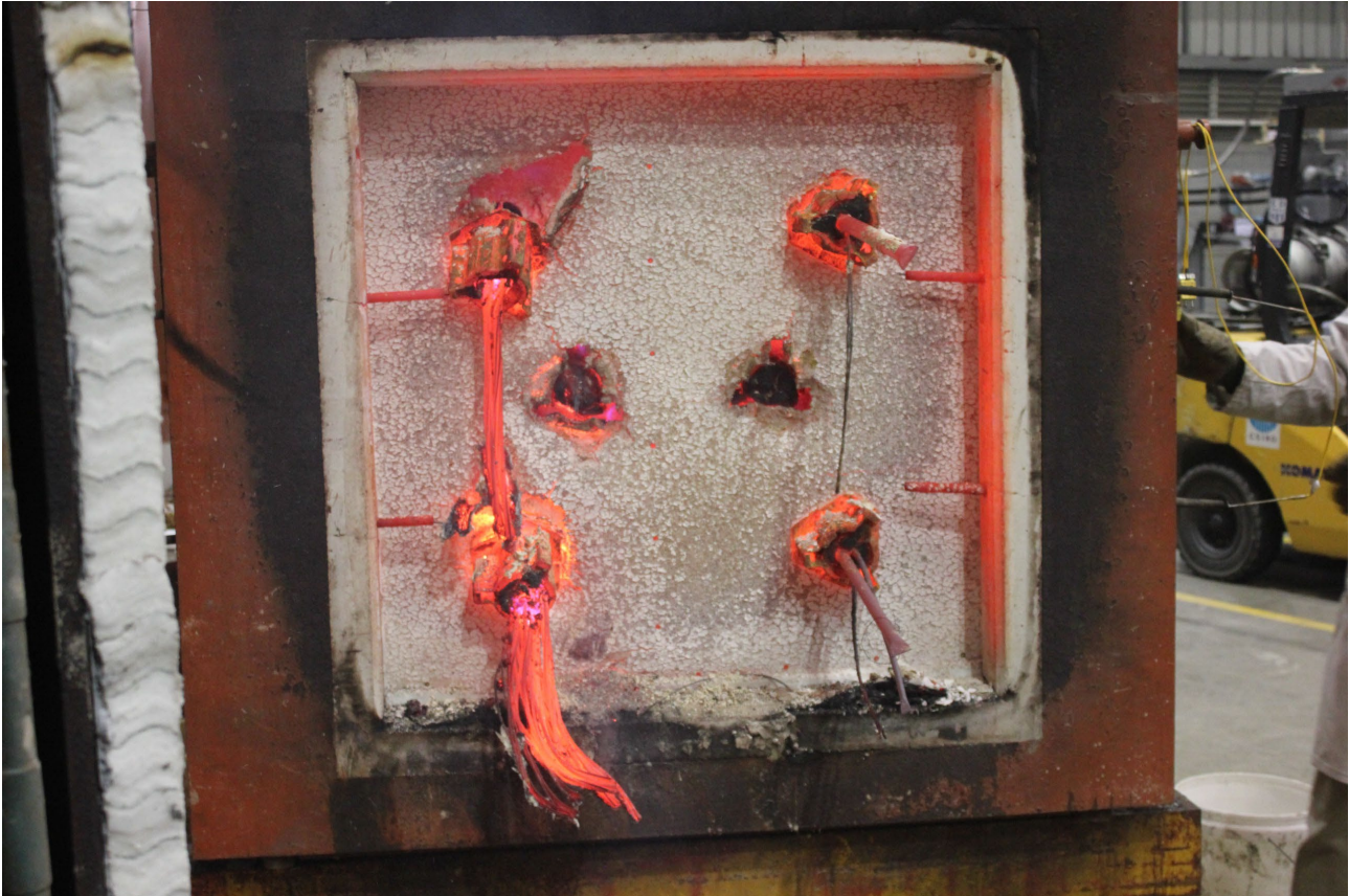
PHOTOGRAPH 12 – EXPOSED FACE OF SPECIMENS AT CONCLUSION OF TESTING
