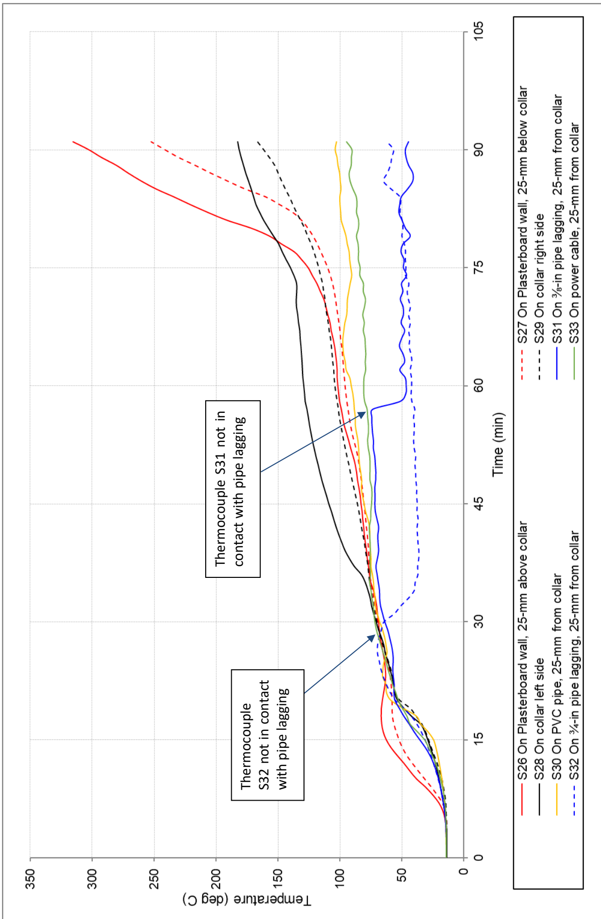
FIGURE 7 - TEMPERATURE VERSUS TIME ASSOCIATED WITH SPECIMEN #5
