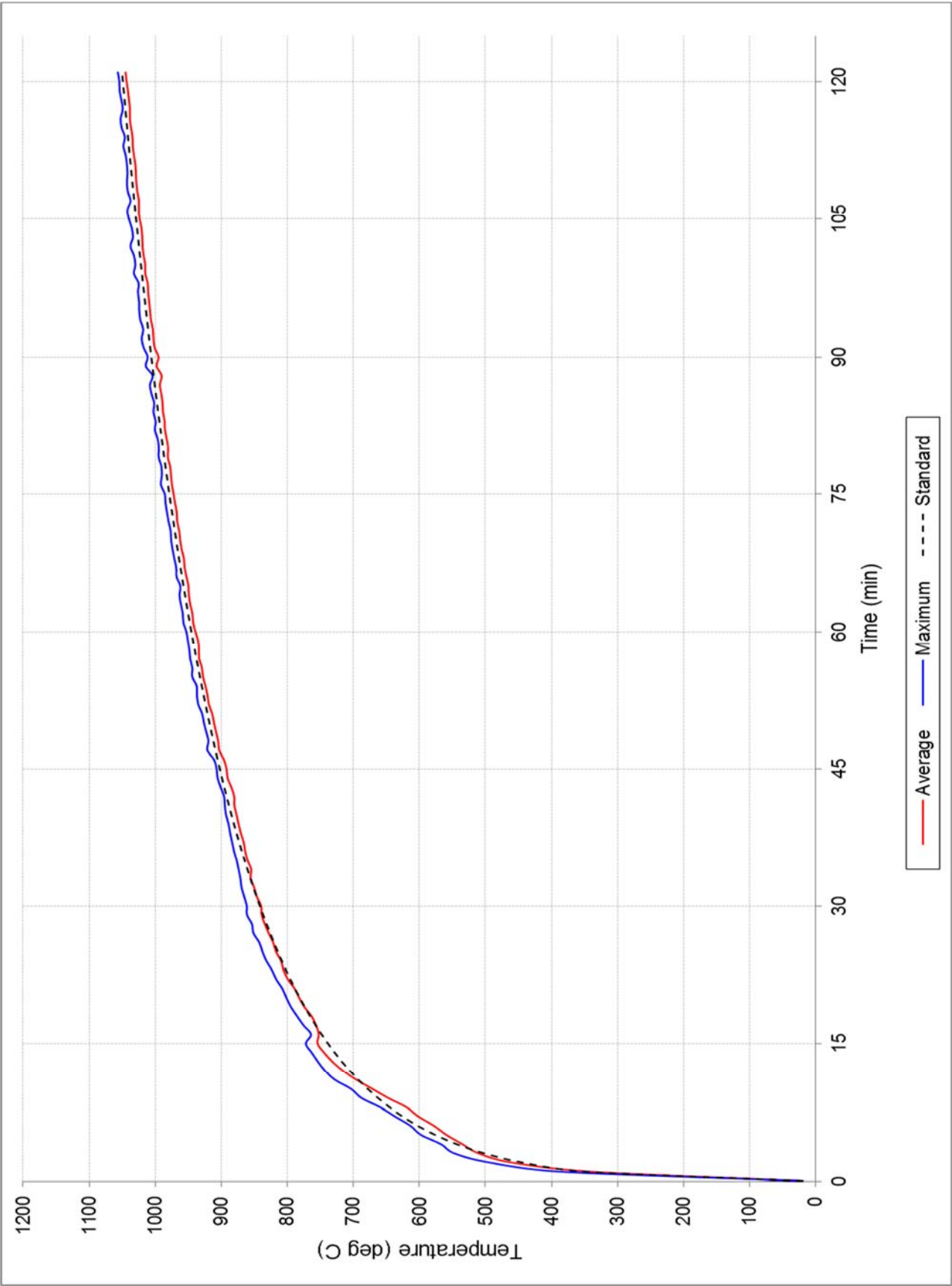
FIGURE 1 – FURNACE TEMPERATURE
