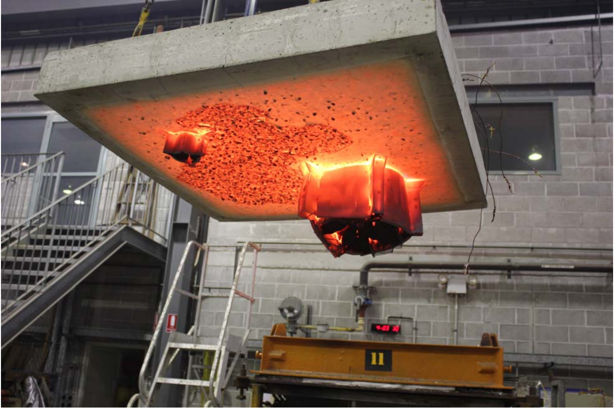
PHOTOGRAPH 9 – EXPOSED FACE OF PENETRATIONS AT CONCLUSION OF TESTING
