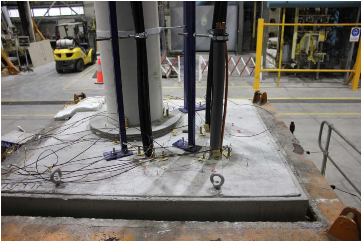
PHOTOGRAPH 2 – UNEXPOSED FACE OF PENETRATIONS PRIOR TO TESTING
