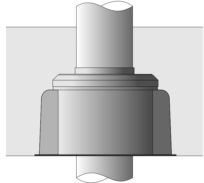
FWS and S models - cast in concrete slab for stack work
