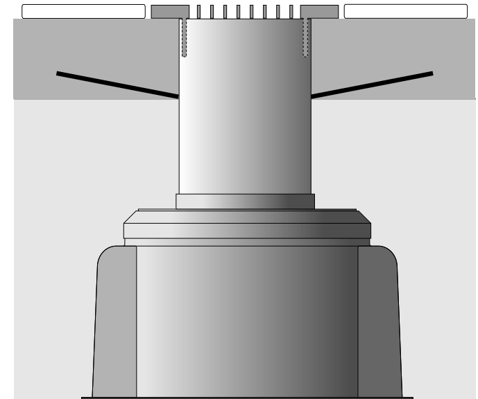
FWS model only - cast in concrete slab with floor waste
